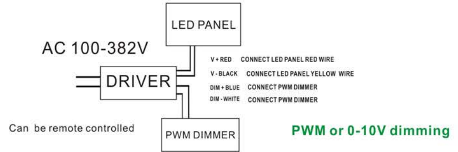
Connection with dimmer
