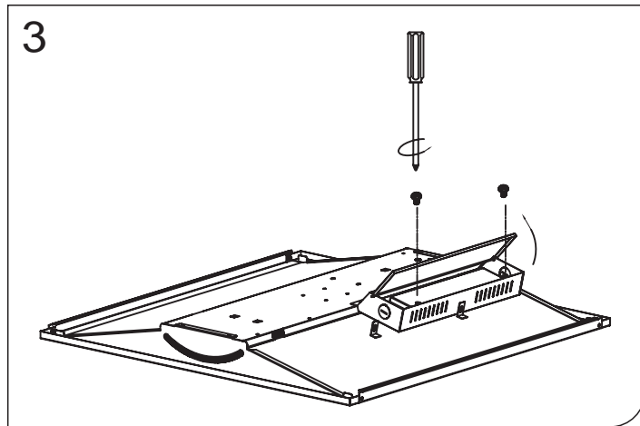
3. Open the terminal block.
