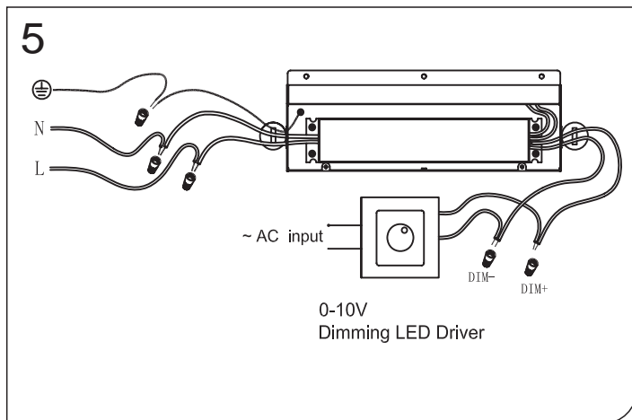
5. Connect dimming wire.
