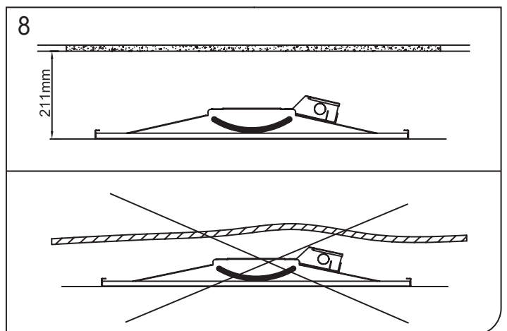
8. Not for use in applications where contact with insulation will occur.
