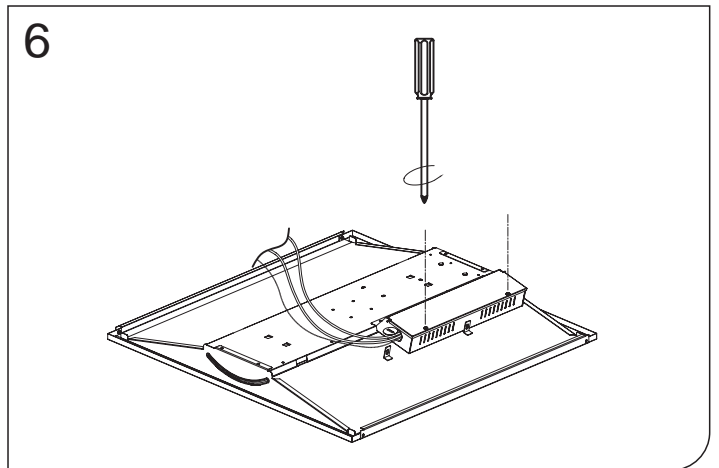
6. After the power cord is correctly connected, reinstall the access plate.
