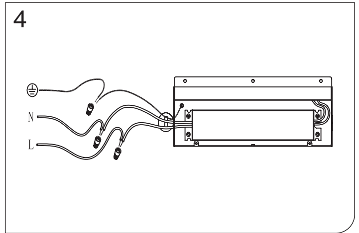
4. Connect the AC wire.
